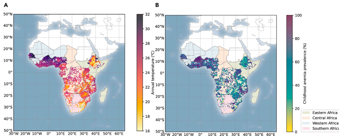
Figure 1. Temperature exposure and prevalence of childhood anemia in sub-Saharan Africa, 2003–2020 (A–B) (A) Annual temperature exposure for studied clusters. (B) Prevalence of childhood anemia for studied clusters in sub-Saharan Africa.
