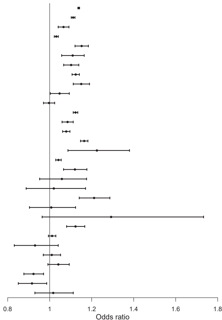
Figure 2. Odds ratios (95% confidence intervals) of childhood anemia per 1°C increase in annual temperature, classified by different regions or countries of sub-Saharan Africa
