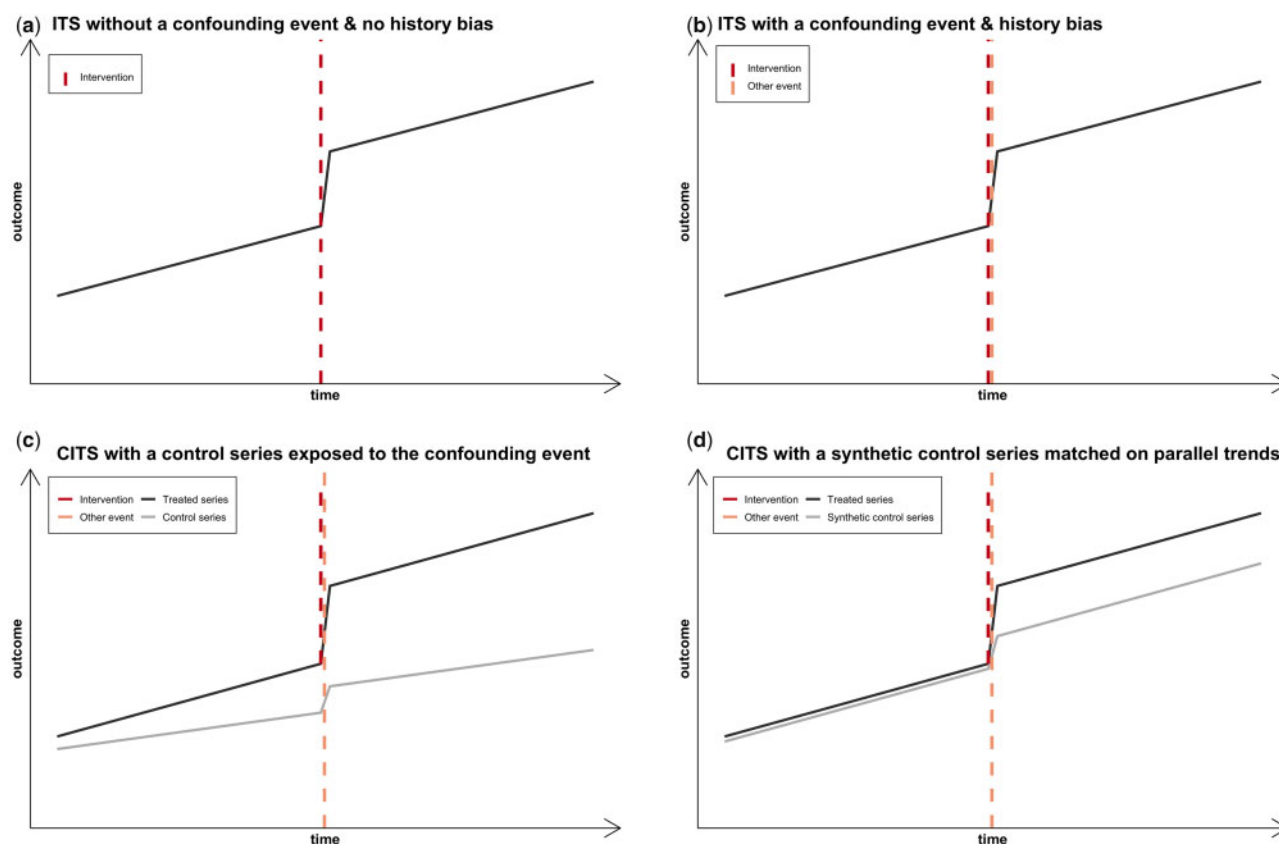
Figure 1 Schematic diagram showing history bias from a confounding other event in interrupted time series designs (simple and controlled). Adapted from Lopez Bernal et al. 12
