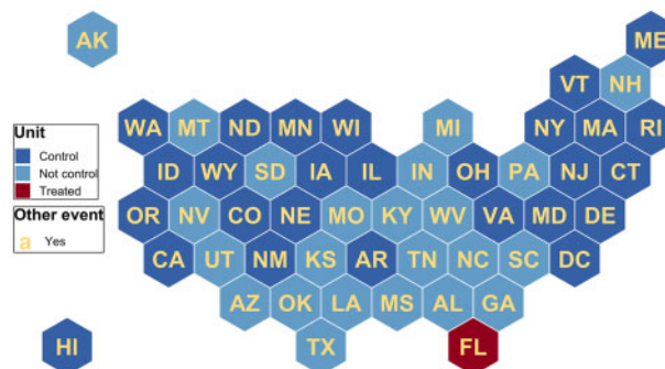
Figure 2 Illustrative example of when the use of synthetic controls in interrupted time series is problematic [state-specific confounding (a)] and beneficial [country-wide confounding (b)]
