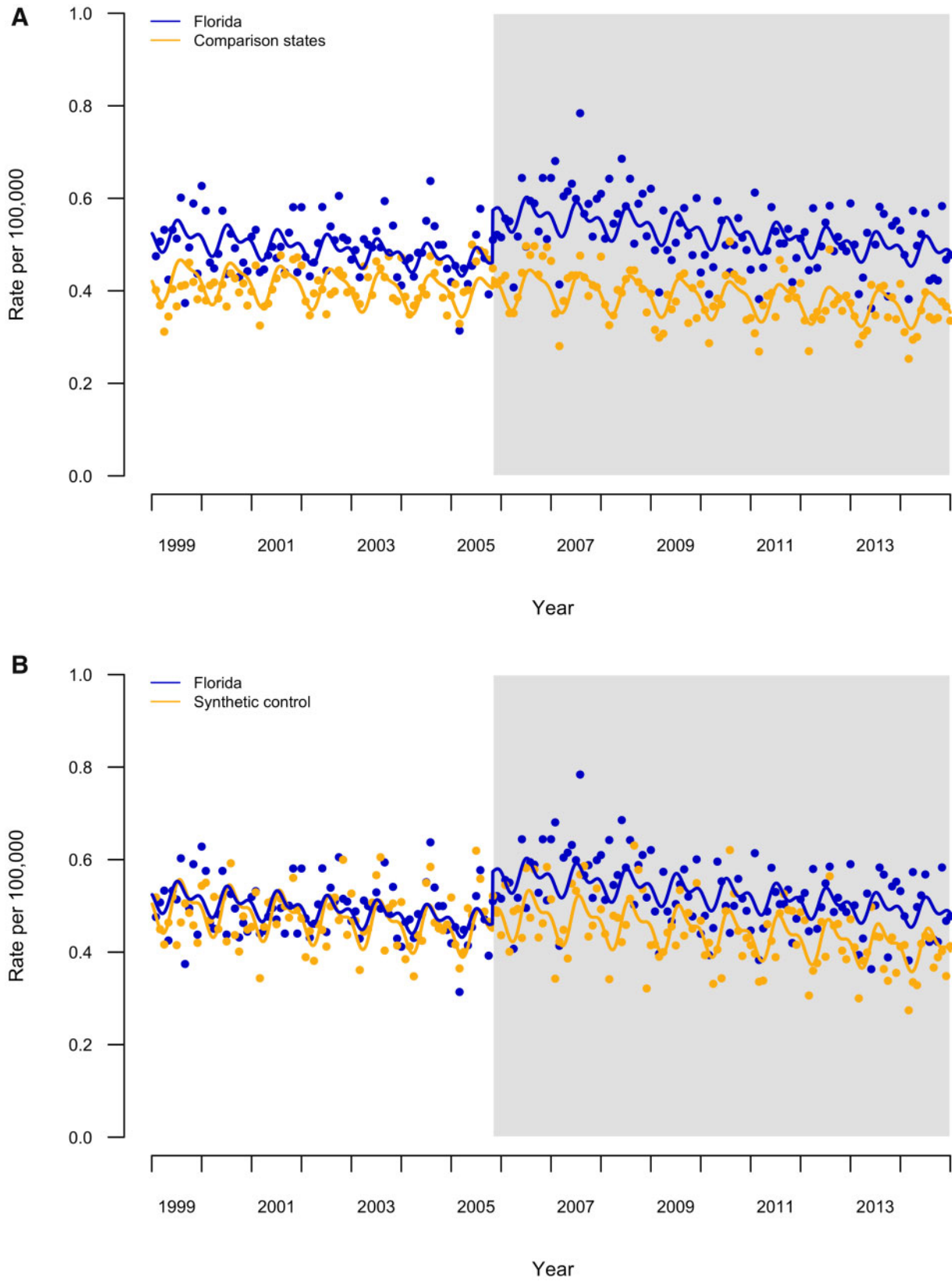
Figure 3 The impact of stand your ground (SYG) law on homicide rates in Florida, 1999–2014, using real data with a USA-wide confounding event: (a) CITS with four comparison states (New York, New Jersey, Ohio, Virginia); (b) CITS with synthetic control (donor pool: 15 comparison states). Adapted from Humphreys et al. (2017) 29
