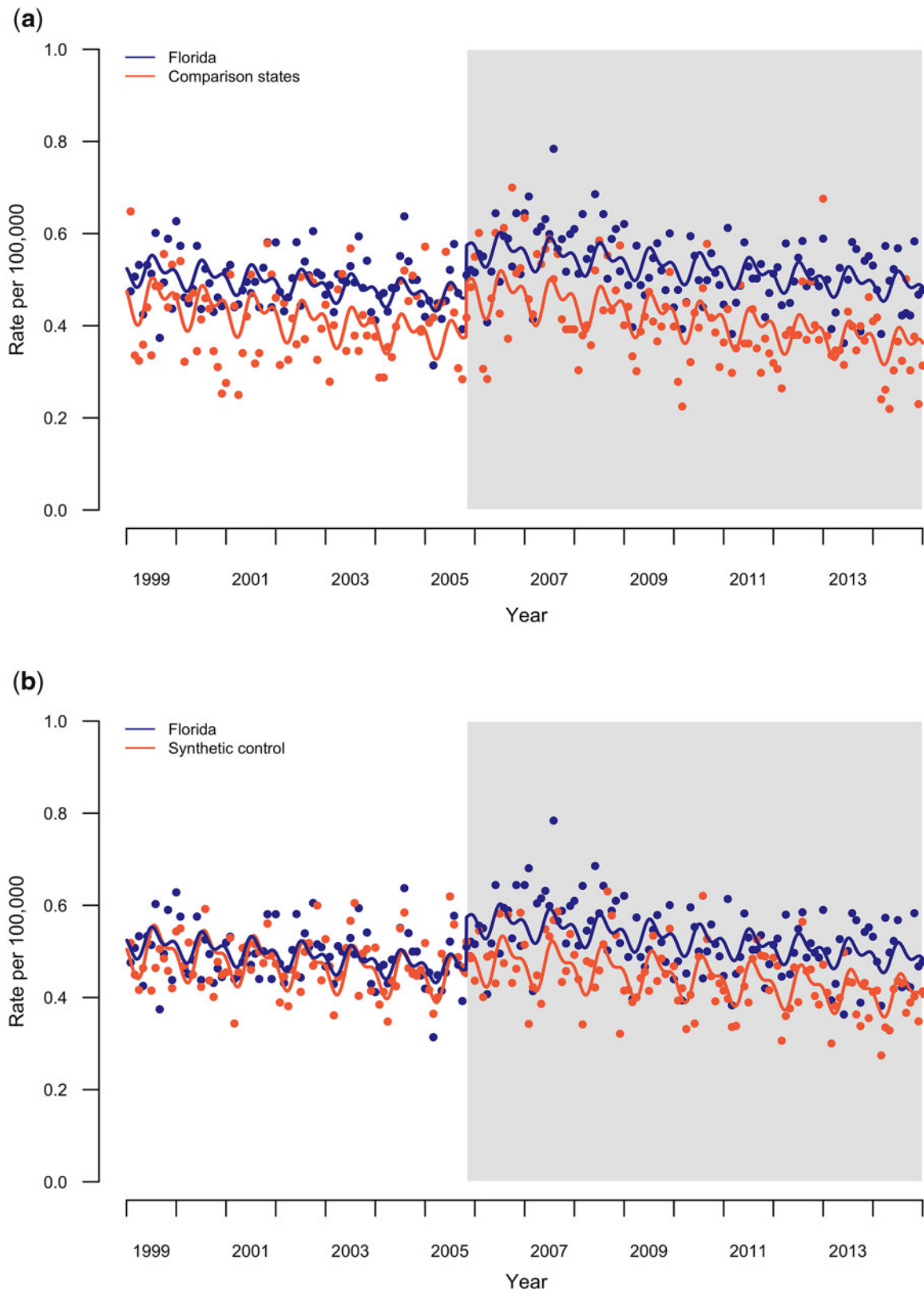
Figure 4 The impact of stand your ground (SYG) law on homicide rates in Florida, 1999–2014, using artificial data with a state-specific confounding event: (a) CITS with two comparison states affected by the confounding event (Maryland, Connecticut); (b) CITS with synthetic control (donor pool: 15 comparison states). Adapted from Humphreys et al. (2017) 29
